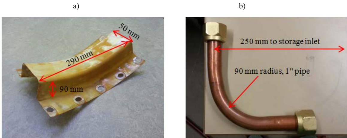
Fig. 9: Inlet flow velocity mitigation plate for inside storage mounting and 90° elbow before the storage inlet
