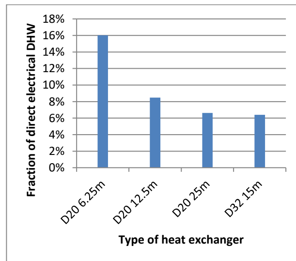
Figure 5: Annual fraction of direct electrical DHW heating with different internal heat exchangers.
