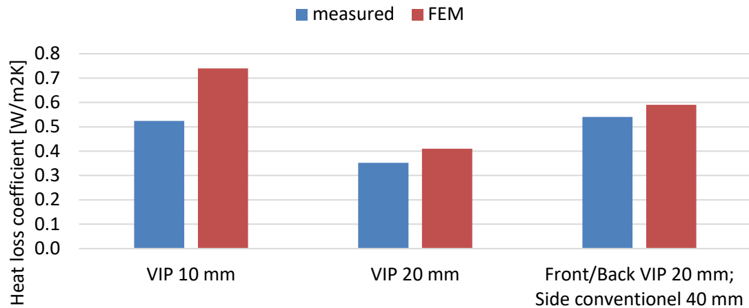
Figure 3: Measured heat loss coefficients vs. the predictions from FEM simulations.
