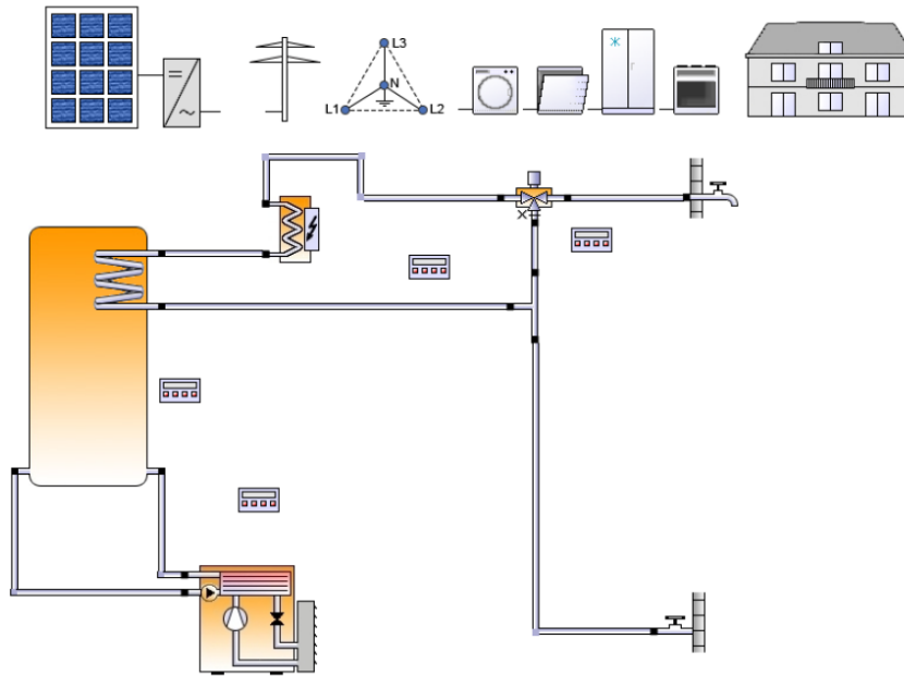
Figure 4: Simulation scheme in the software Polysun.
