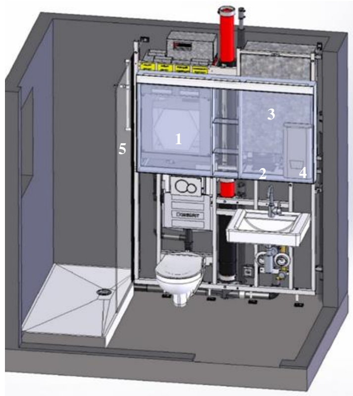
Figure 1: DHW system in the bathroom prewall.
