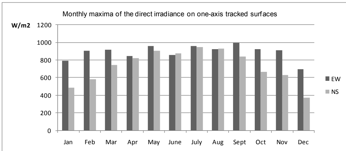
Fig 4: Monthly maxima of the direct irradiance on one-axis tracked surfaces for EW and NS orientation for the location of Fribourg/Switzerland (Swiss midlands, latitude 47°N, longitude 7°E, 588m above sea level).
