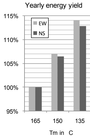
Fig 9: Yearly energy yields of both EW and NS orientated fields for different mean collector temperatures T m , normalized to the yields achieved with T m = 165°C
