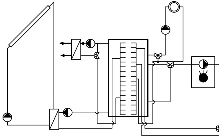
Figure 3: Hydraulic scheme of system test #2. Differing from system test #1, the auxiliary heater is integrated with two three-way valves to switch between the operating modes for DHW-preparation or SH. Again, all volume flows enter the TES through a stratification device.
